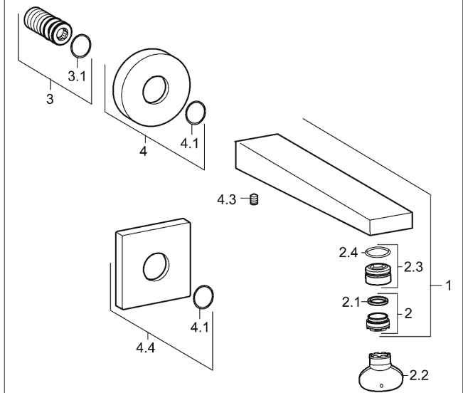
Product Drawing
